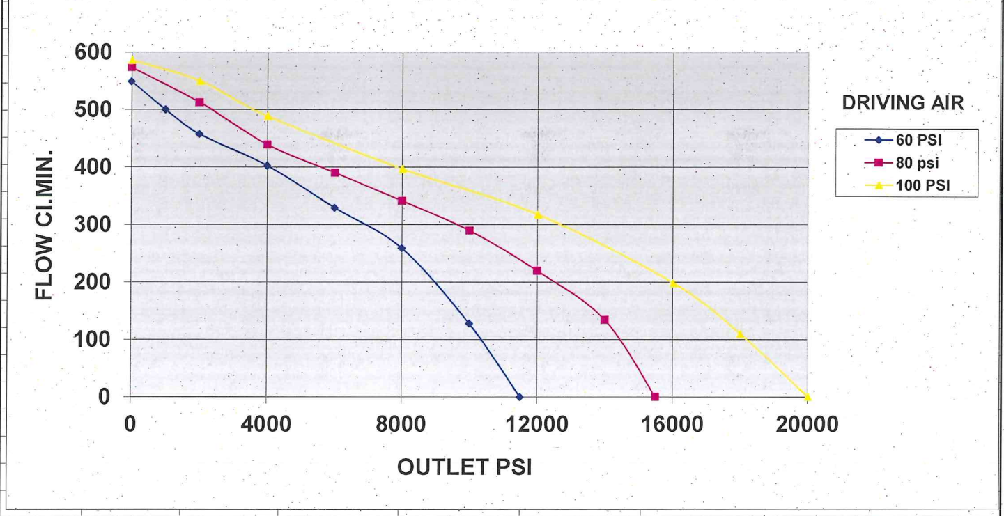
S-218-200D (Double End) #032806J-1 Performance on water (060302J-1) W/Cartridge Pilot Valves
